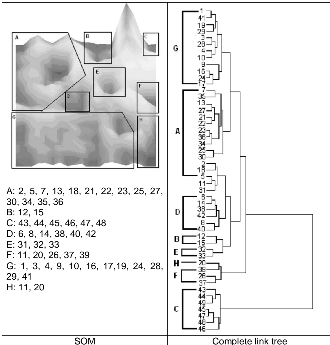
Figure 10: Comparison of SOM and complete link tree clustering
