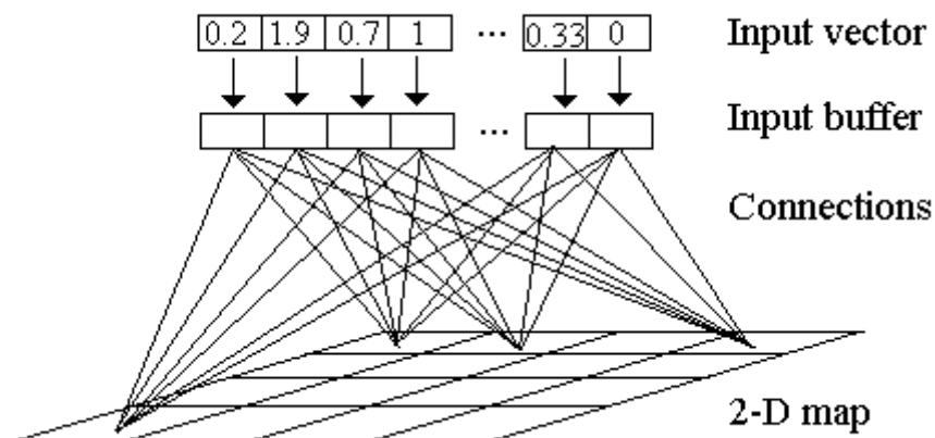
Figure 5: a self-organizing map
