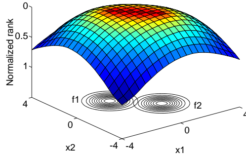
Figure 7: The cost landscape defined by Pareto-ranking
