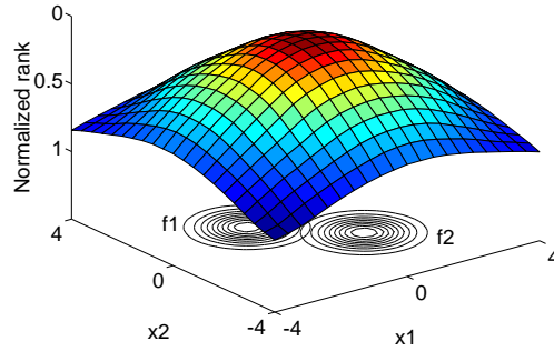
Figure 5: The cost landscape defined by ranking objectives separately and averaging the ranks
