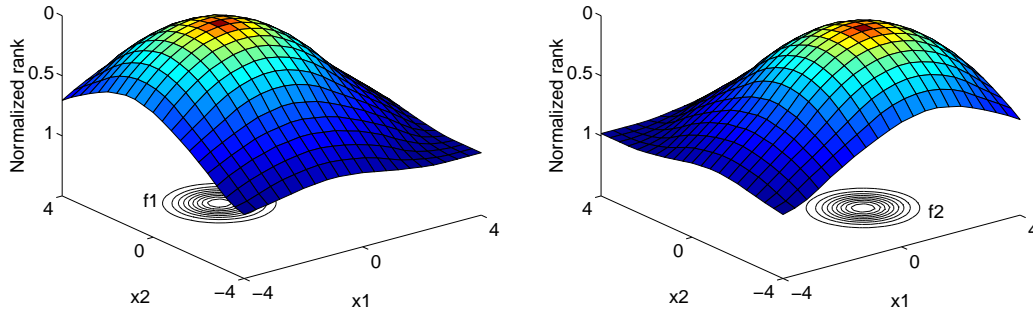
Figure 3: The cost landscapes defined by ranking each objective separately (and contour plots of the corresponding objective functions)
